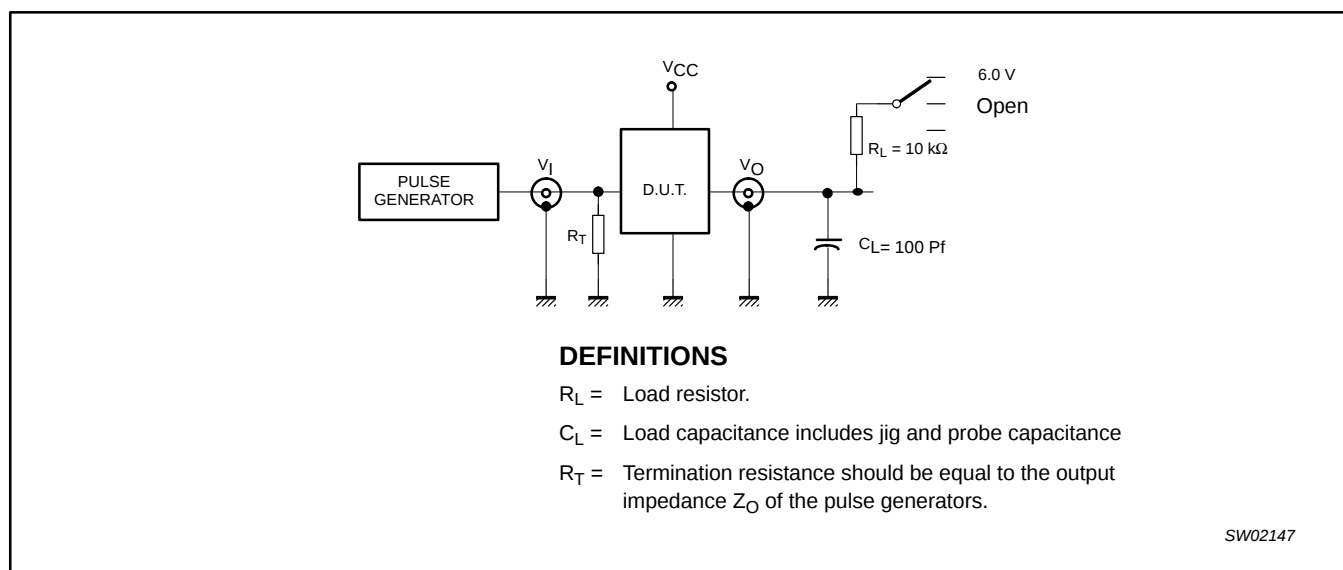
Figure 19. Test circuitry for switching times
