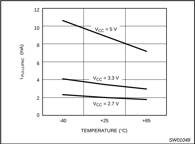
Figure 13. I PULLUPAC versus Temperature.
