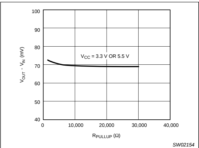
Figure 15. Connection circuitry V OUT - V IN .
