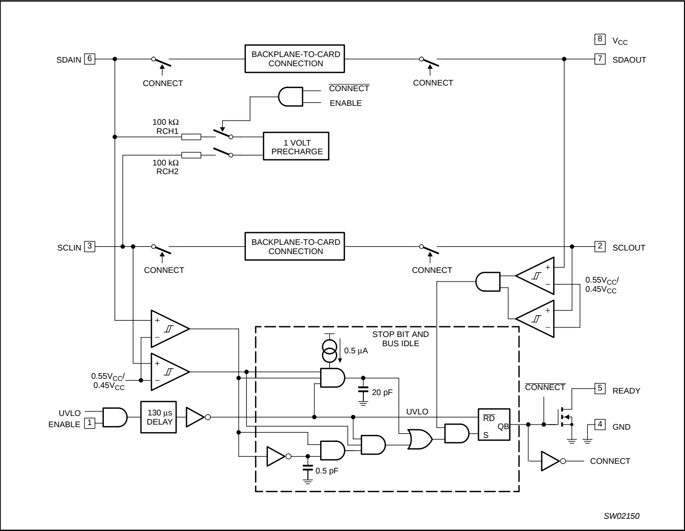
Figure 3. Block diagram — PCA9510
