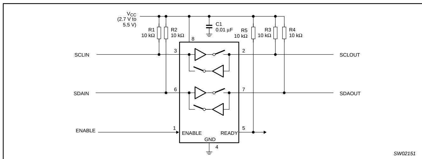
Figure 4. Typical application — PCA9511
