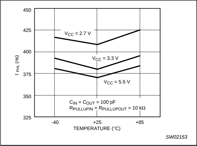
Figure 14. Input-output t PHL versus Temperature.
